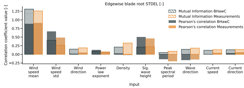
(a) Blade edgewise 10-min. DEL
